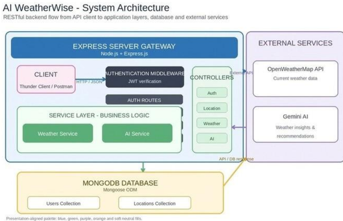
Figure 6.1: System Architecture of AI WeatherWise
